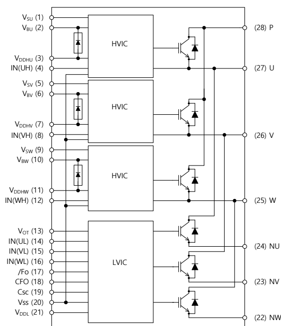
Figure 1. Internal Circuit
