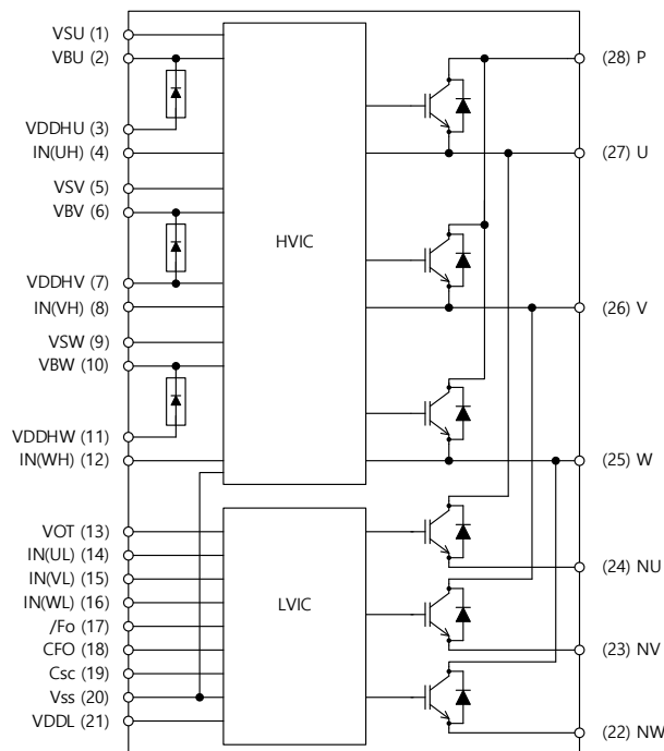
Figure 1. Internal Circuit
