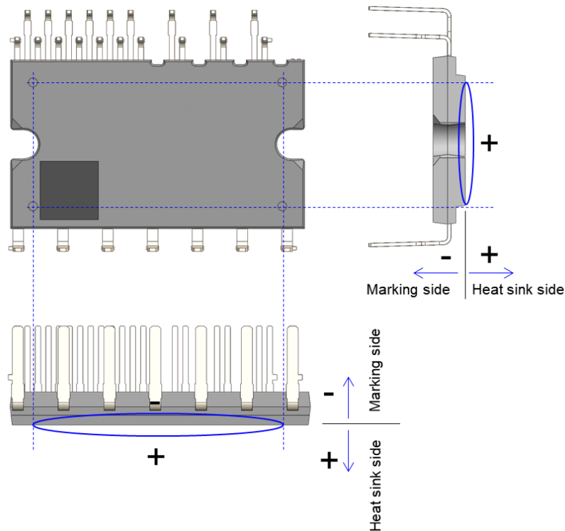
Figure 8. Flatness Measurement Position
