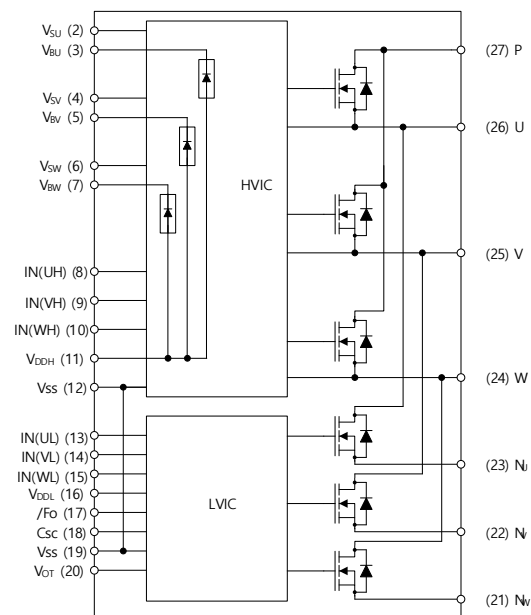
Figure 1. Internal Circuit
